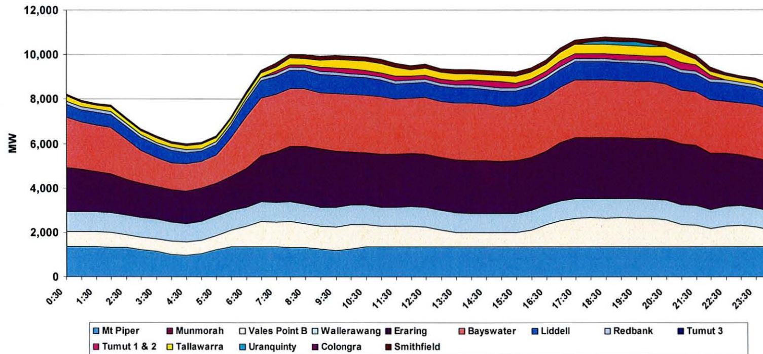
Electricity Generation by Major Plants in NSW 15 June 2011
