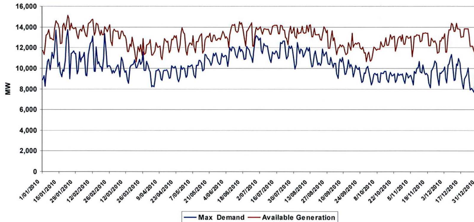
New South Wales Maximum Demand and Available Generation 2010 Calendar Year
